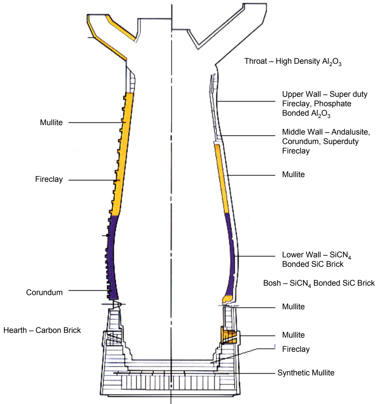
TYPICAL BLAST FURNACE
